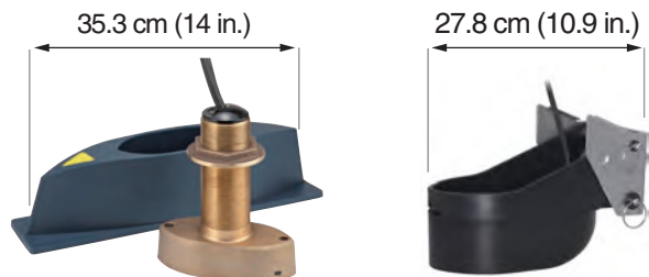
Thru-hull mount transducer B54 or SS54 Transom mount transducer TM54
